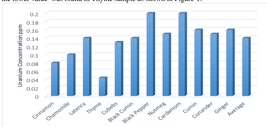
Figure 1- Uranium concentrations in herbal plants samples
