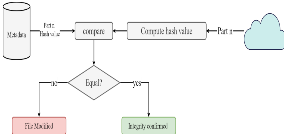
Figure 4 Integrity checking
