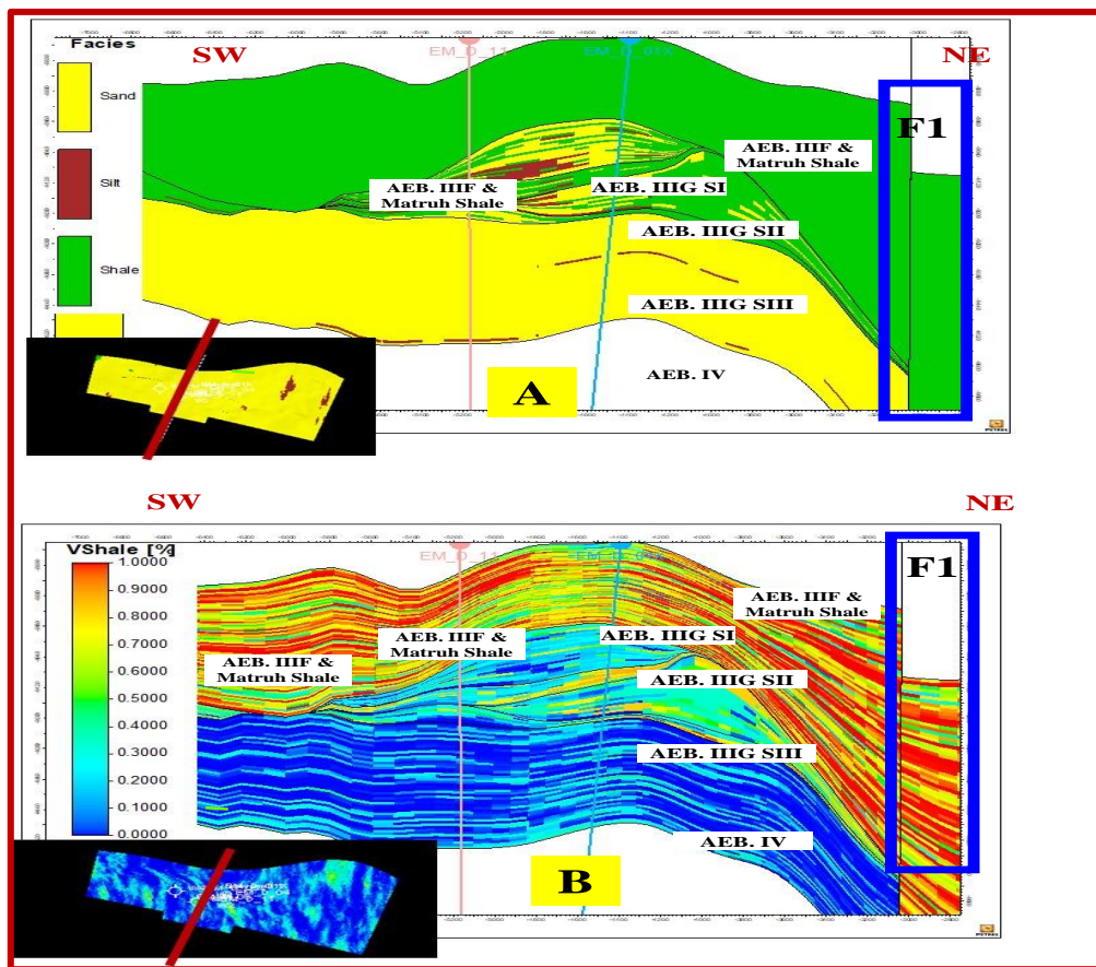
Figure 12: Cross section for (Litho-facies) and (Vsh) of the Alamein Formation to Alam El Bueib IIIG target fault No. 1 (F1).
