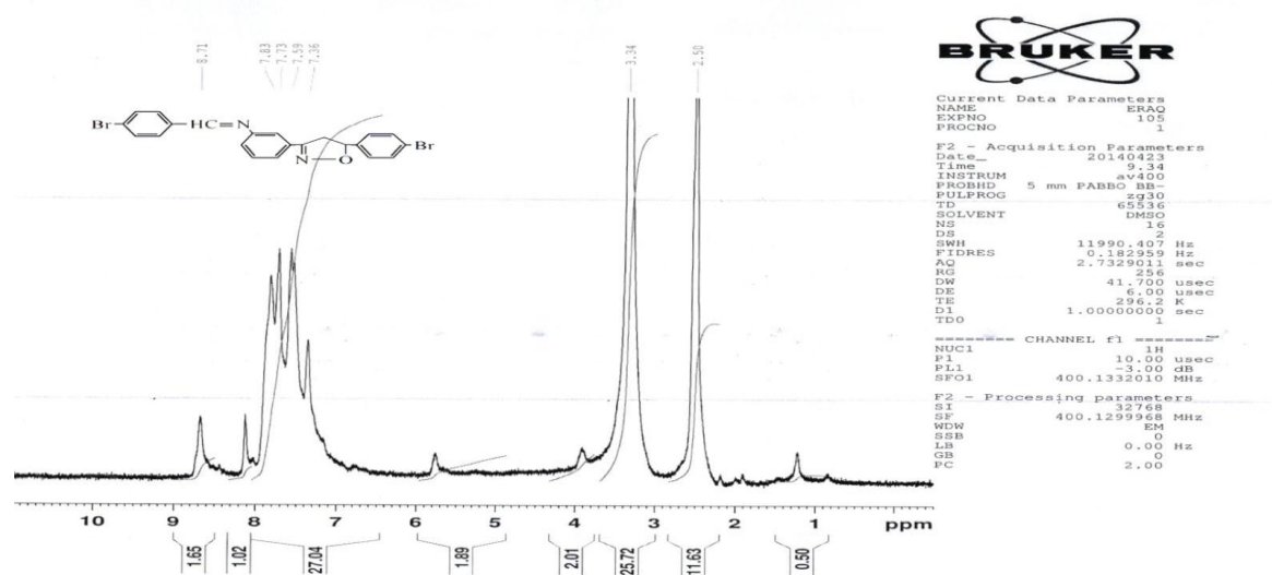
Figure 1- 1 H-NMR-Spectrum of compound (IV) b
