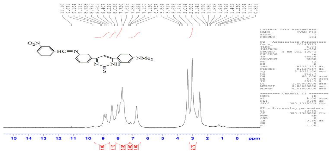
Figure 2- 1 HNMR-Spectrum of compound (V) d
