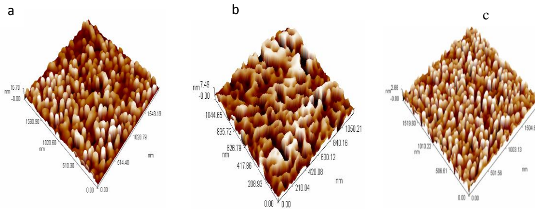
Figure 2- 3D AFM image of Au NPs with (a) 200, (b) 360, and (c) 500 m J.
