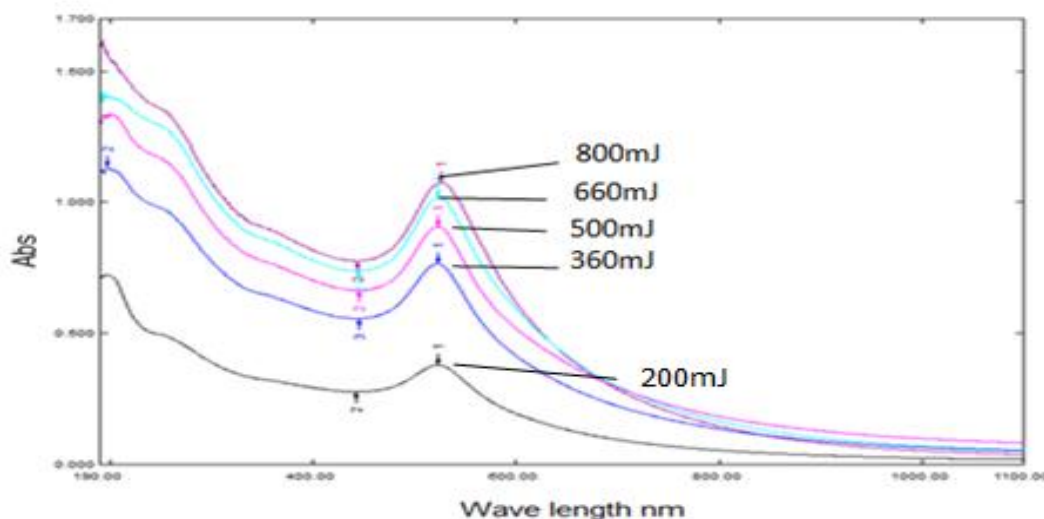
Figure 1- Absorption spectra of Au NPs.
