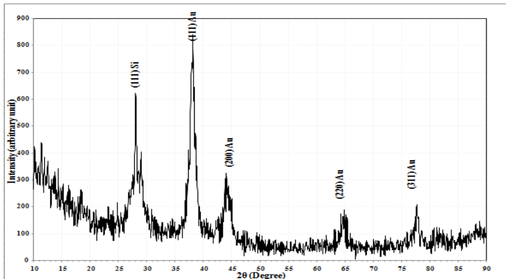
Figure 3- X-ray diffraction pattern of Au NPs at laser energy 800 mJ/pulse.
