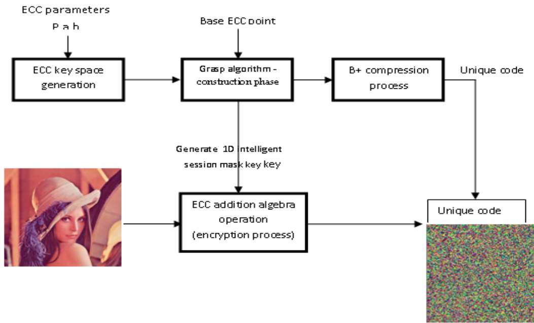
Figure 2- The proposed approach to generate the secret session intelligent mask and sending process
