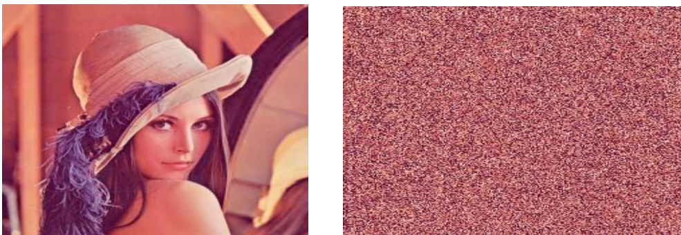
Figure 4a- Original and encrypt lena image size (256×256).
