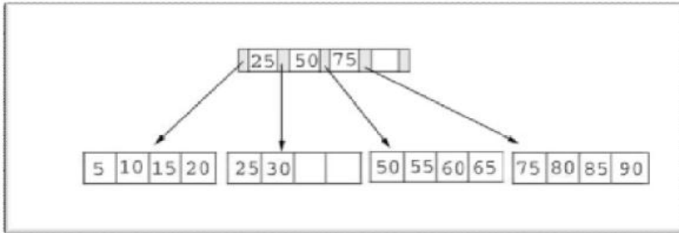
Figure 1- B + Tree example.
