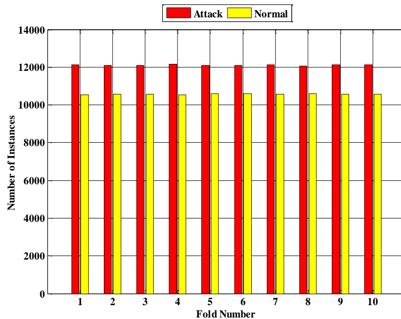
Figure 1- Total number of normal and attack instances for each fold in the training dataset.
