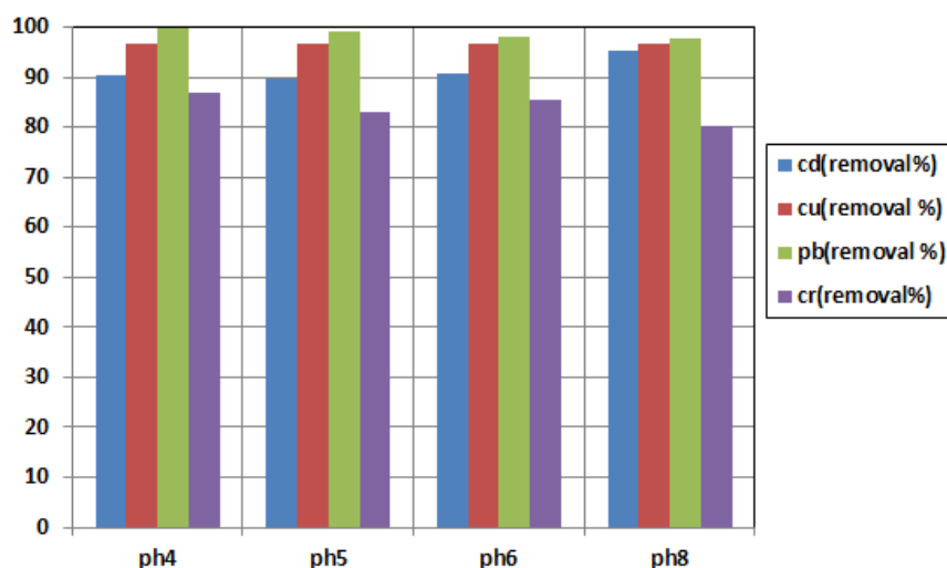
Figure 1 -Effect of variable pH values on the removal of heavy metals by E.crassipes (adsorbent Biomass: 1g, HM: 1000 ppm, pH range 4, 5,6and 8)
