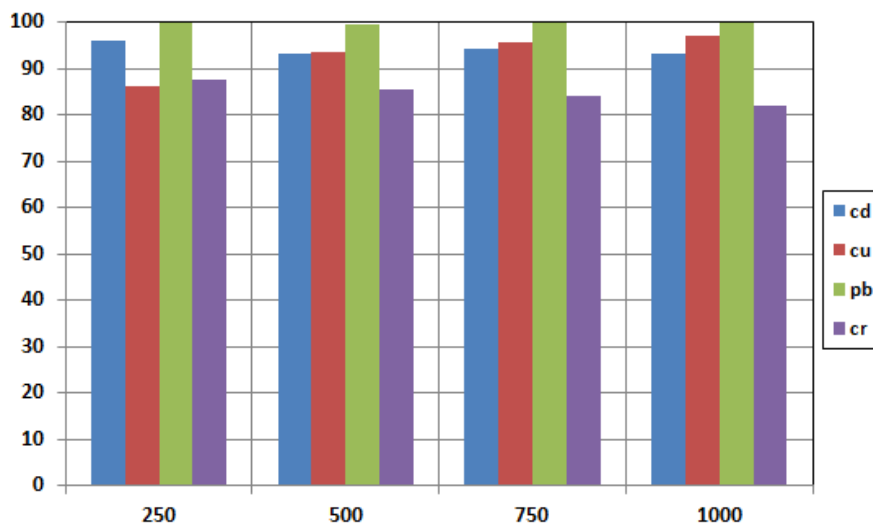
Figure 2- Effect of concentration on the removal of heavy metal by E.crassipes (adsorbent dosage: 1g, HM: 250, 500, 750 and 1000 ppm, pH=7).
