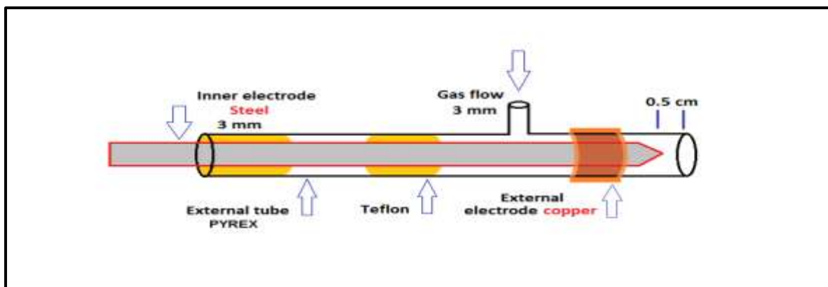
Figure1- Schematic for design non thermal argon plasma needle.
