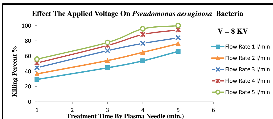
Figure 4- The effect of the non-thermal argon plasma needle on bacteria Pseudomonas aeruginosa at 8 kV and distance 2cm at different flow rate.
