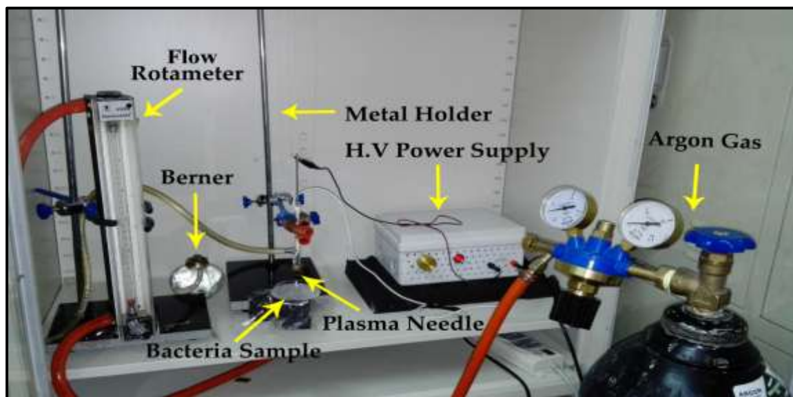
Figure 2- the non-thermal plasma needle system.
