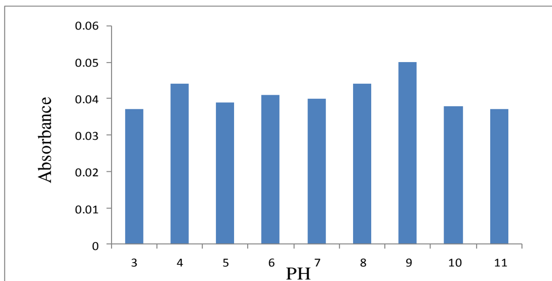
Figure 3-6- Effect of pH on the formation of Pt (IV)-4-AAP complex.
