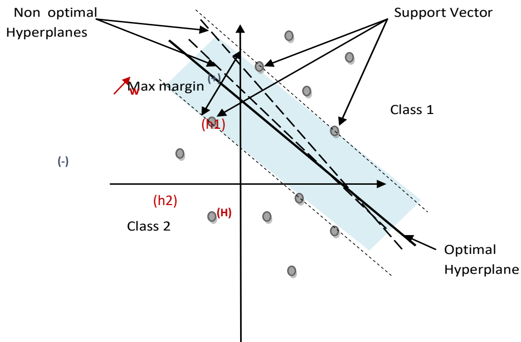
Figure 1-Hyperplane separating data belonging to two classes
