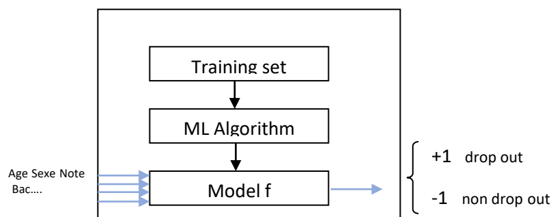
Figure 6 -Formalization problem
