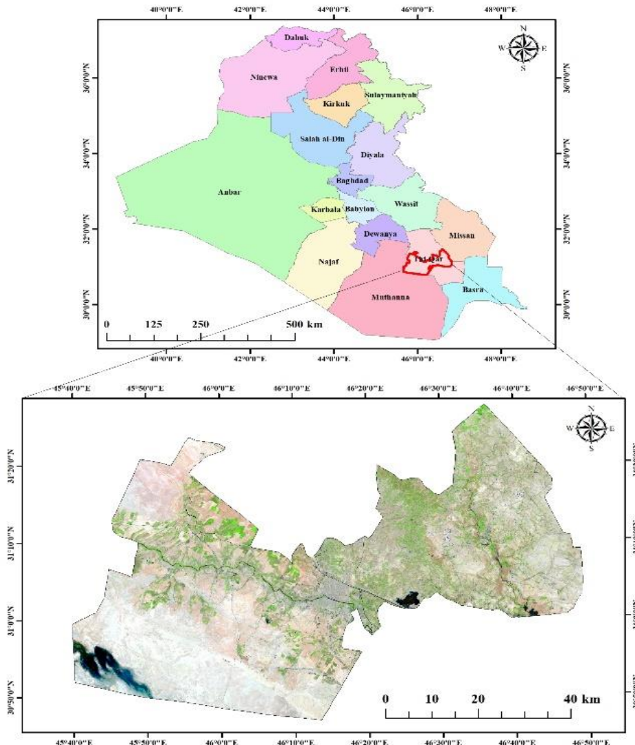
Figure 1: Nasiriya District's location inside the Dhi Qar province by Landsat 9-OLI2 image
