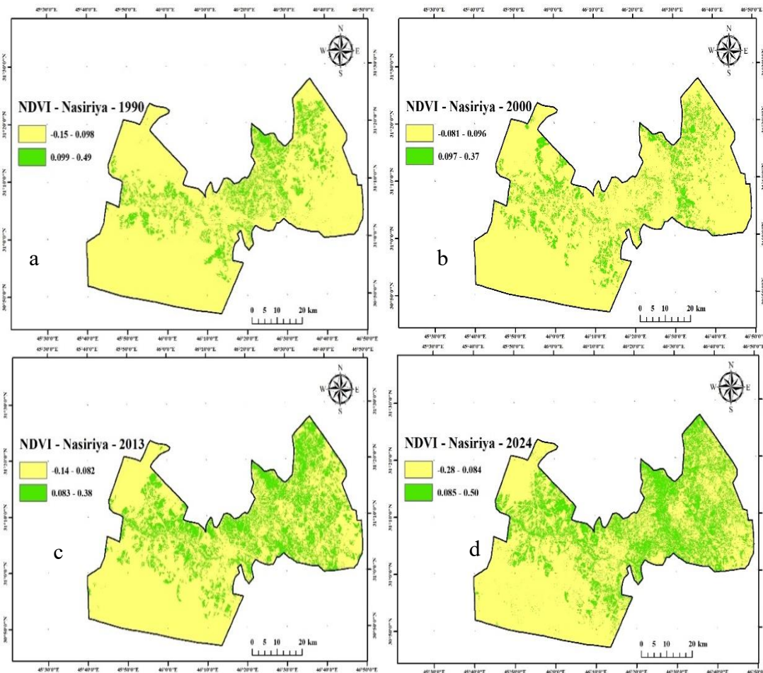
Figure 3: NDVI of Nasiriya district in (a) 1990, (b) 2000, (c) 2013, and (d) 2024
