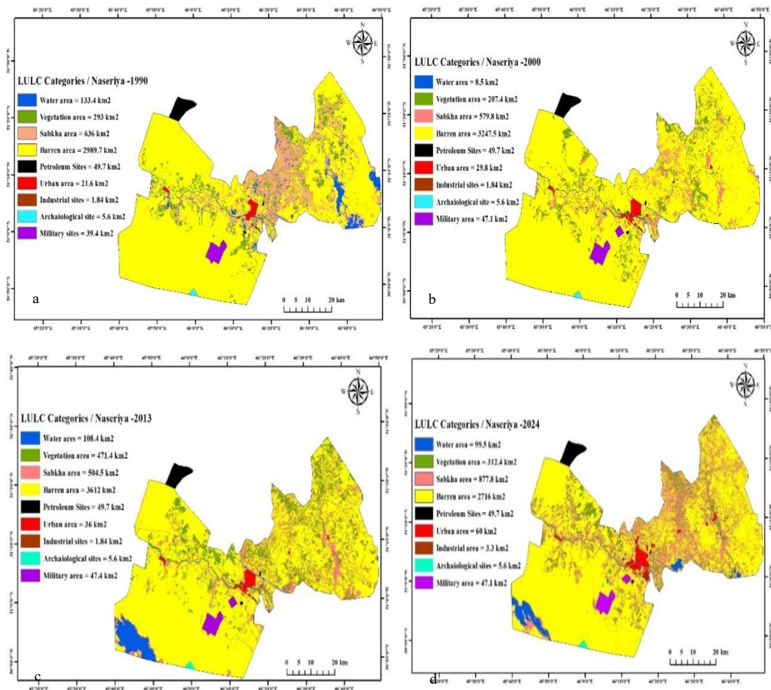
Figure 5: LULC analysis of Nasiriya district
