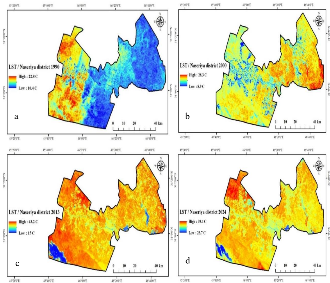
Figure 6: LST values in Nasiriya District, a 1990, b- 2000, c- 2013, d- 2024
