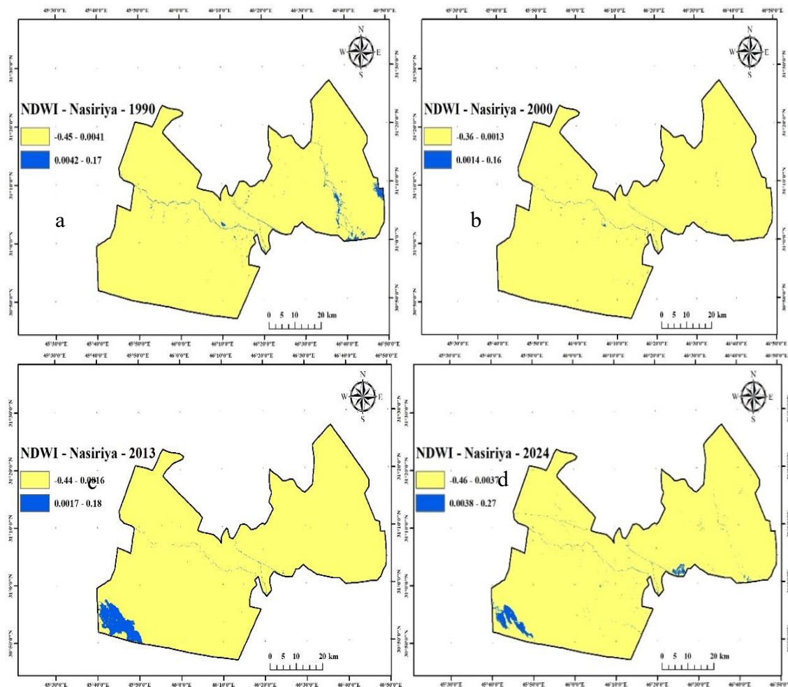
Figure 4: NDWI of Nasiriya district in (a) 1990, (b) 2000, (c) 2013, and (d) 2024
