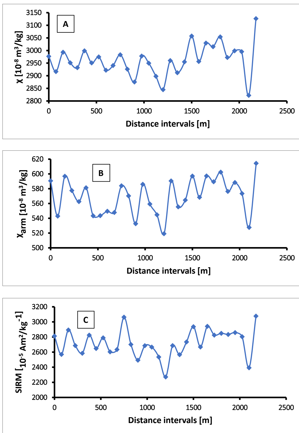
Figure 2: profiles of A) magnetic susceptibility ( \chi ); B) Anhysteretic remanent magnetisation ( \chi_{\text{ARM}} ); C) Saturation isothermal remanent magnetisation (SIRM) versus distance intervals of sediment samples collected from the Tigris River, Baghdad City.
