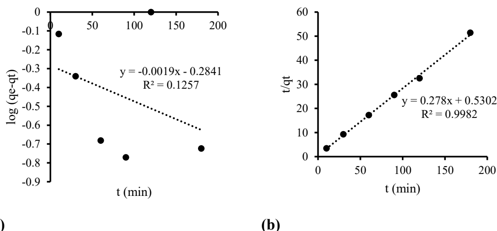
Figure 11: (a) pseudo-first-order and (b) pseudo-second-order kinetic models
