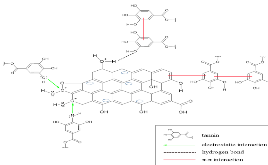
Figure 13: Possible multilayer interaction of tannins with AC-CBW
