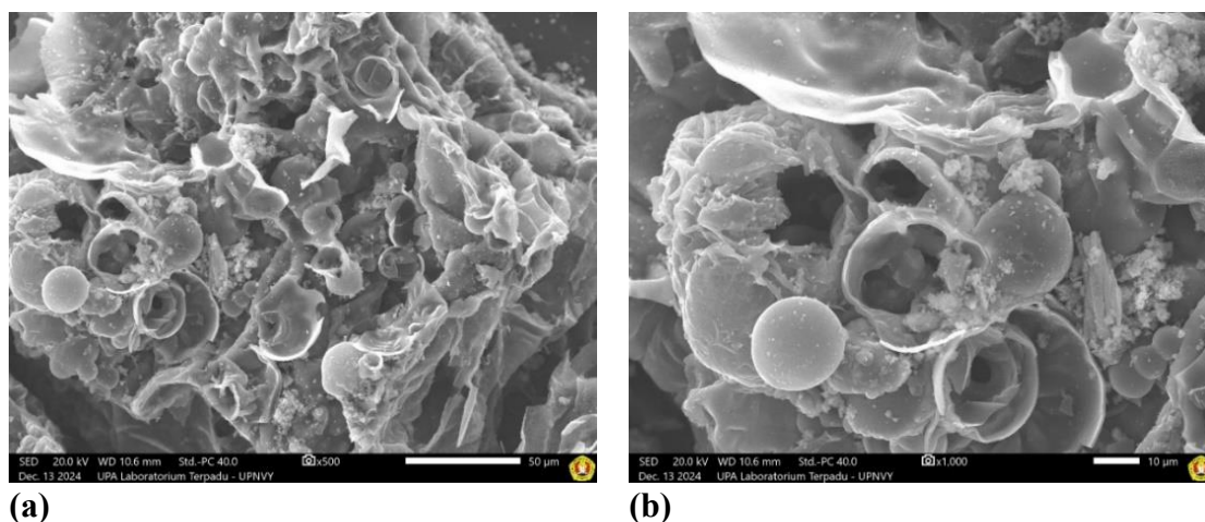
Figure 3: SEM images of C-CBW magnification (a) 500× and (b) 1000×
