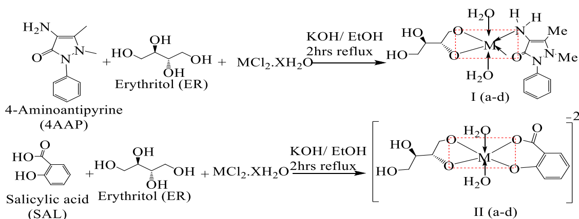
Scheme (1): The synthetic routs of the designed new complexes I and II
