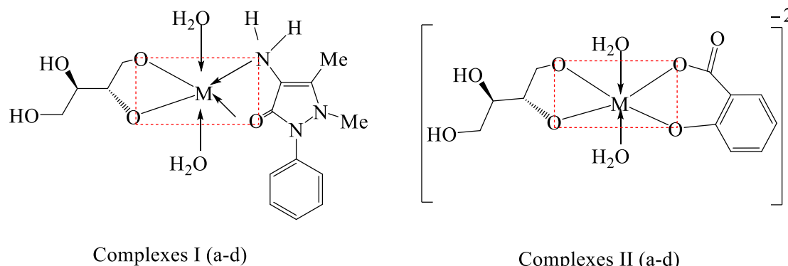
Scheme (2): The general chemical structures of new compmlxes I(a-d) and II(a-d)
