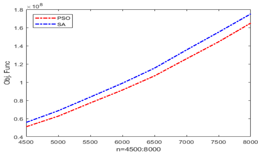
Figure 4 : Comparison results of PSO and SA for problem ( BO – SCLm ), for n = 4500:500:8000 .
