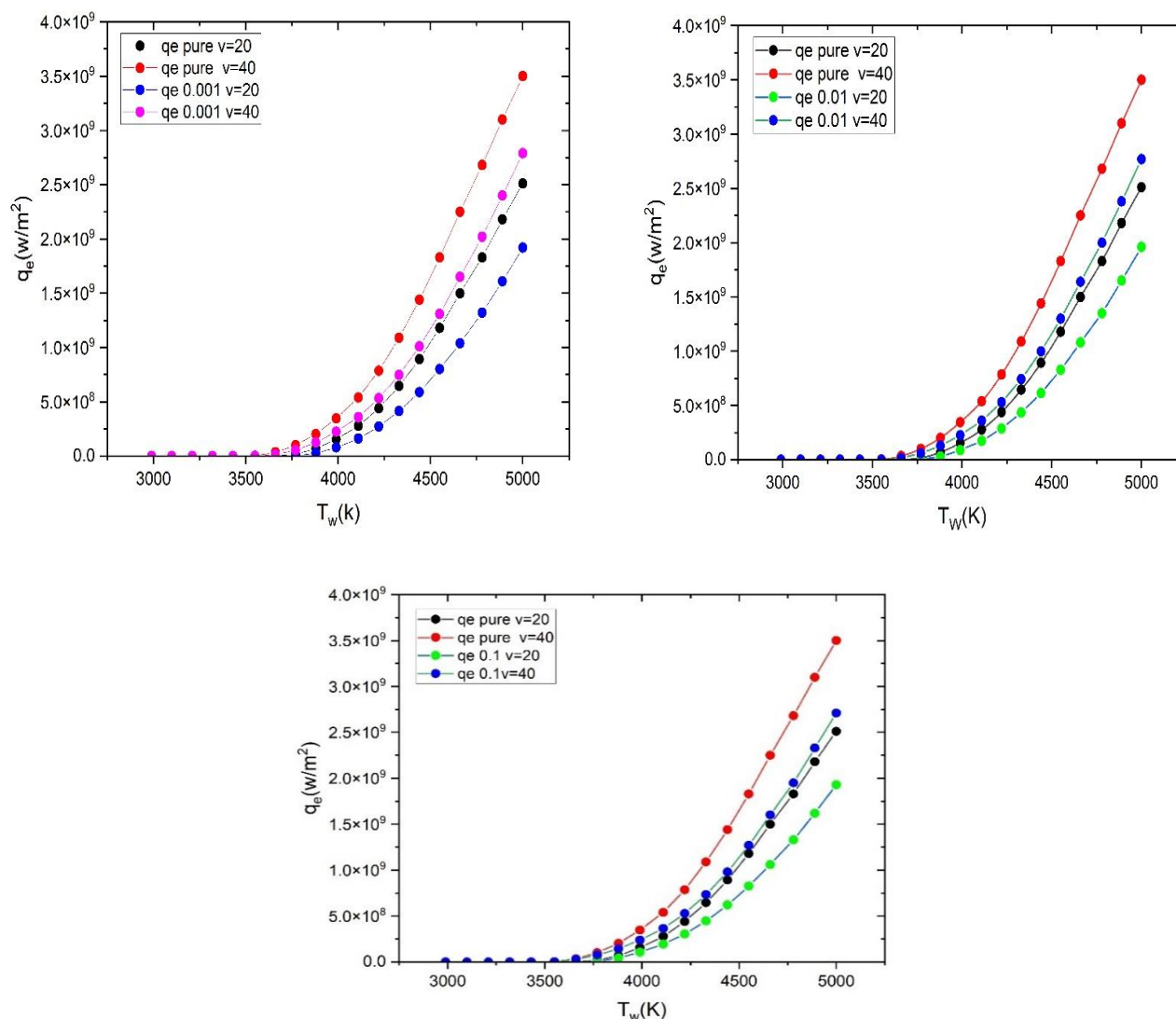
Figure -5: The electron energy flux ( q_e ) using pure xenon and xenon–thallium gas mixture at thallium concentrations of (0.001, 0.01 and 0.1 mol.) vs. the cathode surface temperature T_w at U= 20 V and 40V.
