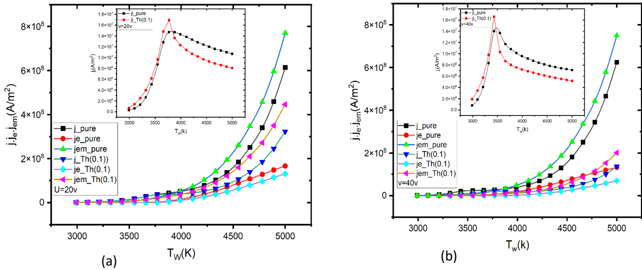
Figure -4: Current density j, j_e, j_i and j_{em} vs. cathode temperature for pure xenon and xenon–thallium gas mixture at 0.1 mol thallium concentration at (a): U=20 V and (b): U=40 V
