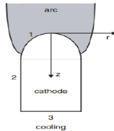
Figure -1: High-pressure arc plasma heating system for heat-resistant cathodes [4].
