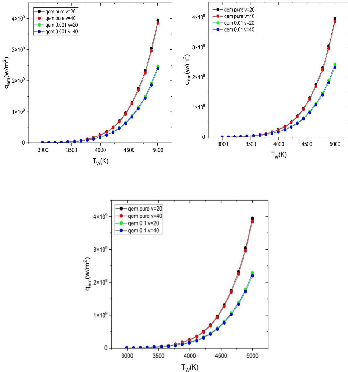
Figure -6: The electron energy emitted from cathode surface ( q_{em} ) using pure xenon and xenon–thallium gas mixture at thallium concentrations of (0.001, 0.01 and 0.1 mol.) vs. the cathode surface temperature T_w at U= 20 V and 40 V.
