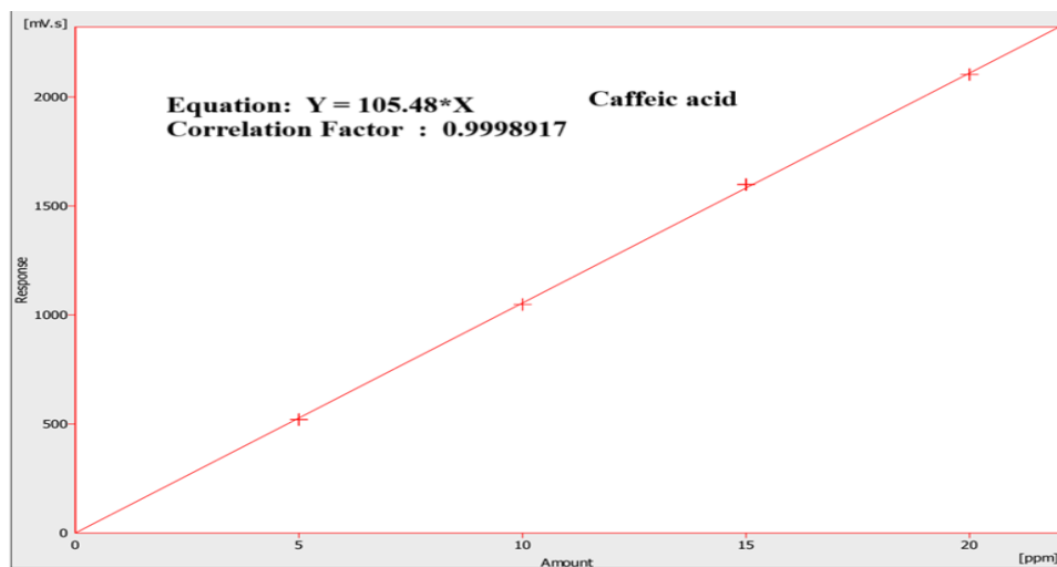
Figure 9: Calibration curve of caffeic acid standard.
