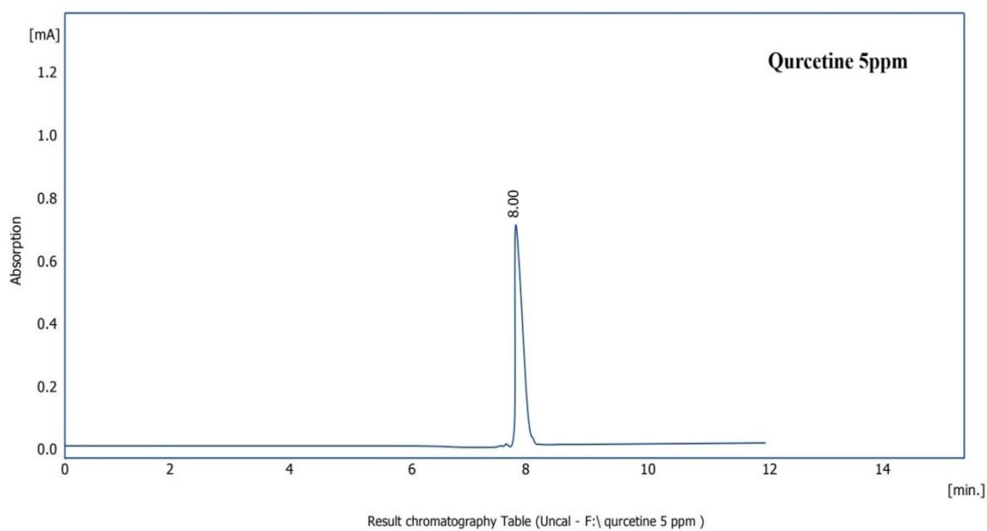
Figure 3: HPLC chromatograms of quercetin standard.
