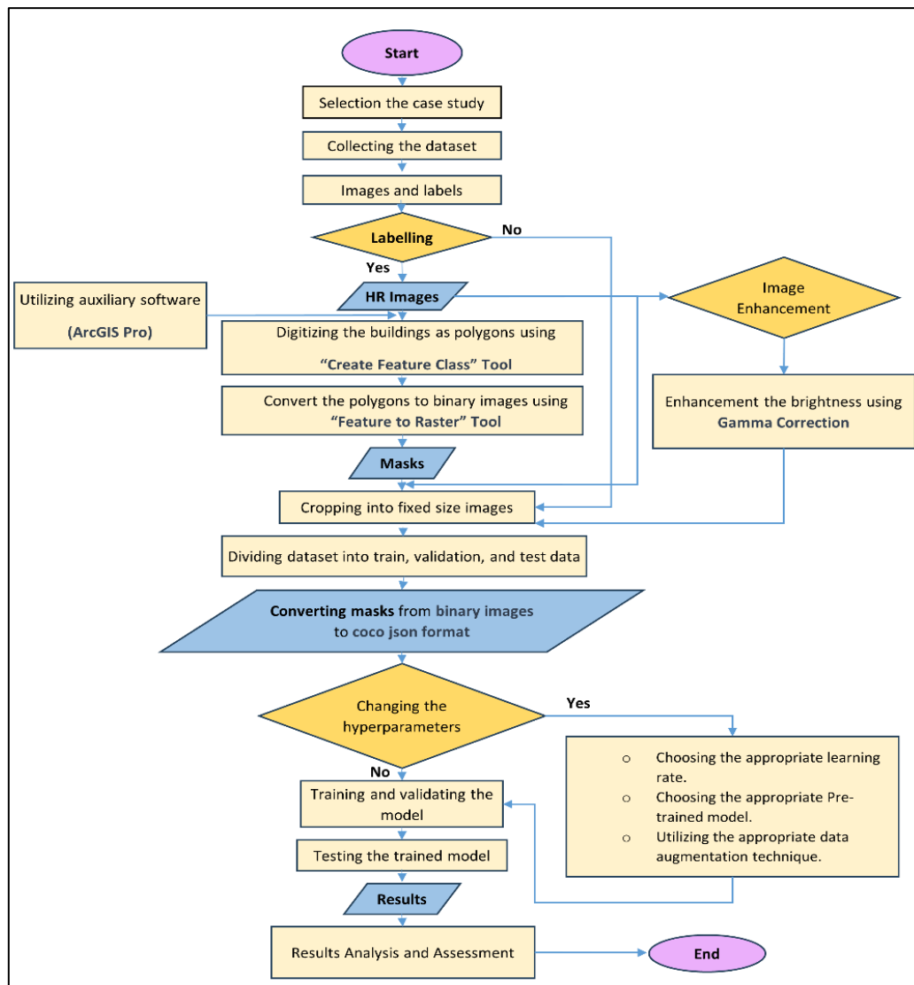
Figure 1: The Flow chart of the implemented methodology.
