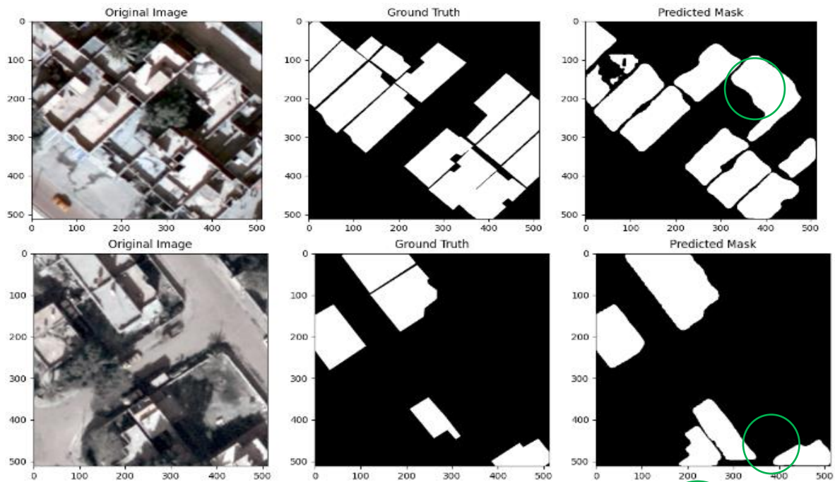
Figure :7 Samples showing the Model's efficiency in extracting buildings using the Baghdad dataset.
