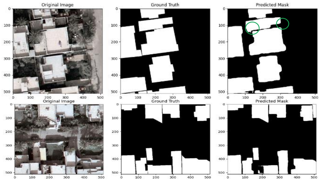
Figure 9: Samples of shadow effects in AL-Mansour and AL-Karrada districts.
