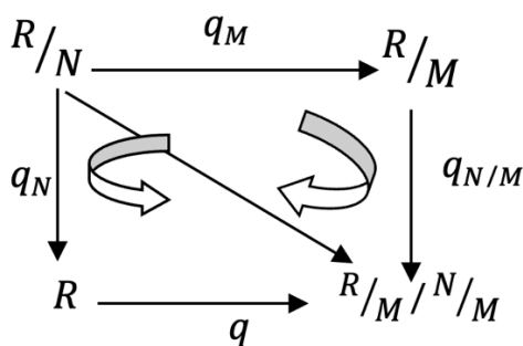
Figure 3: Topological ring groupoid
