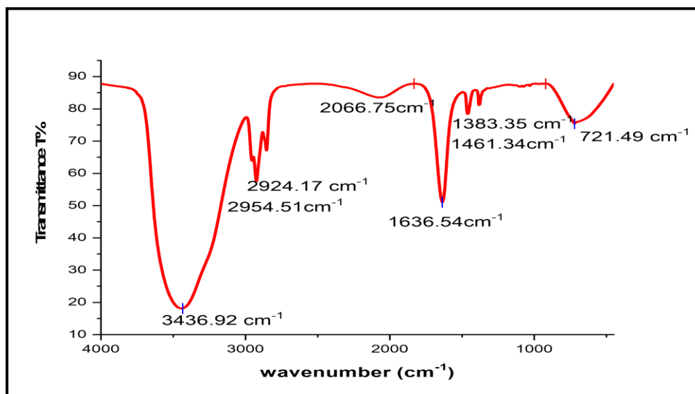
Figure 6: FTIR of Fe 3 O 4 NPs
