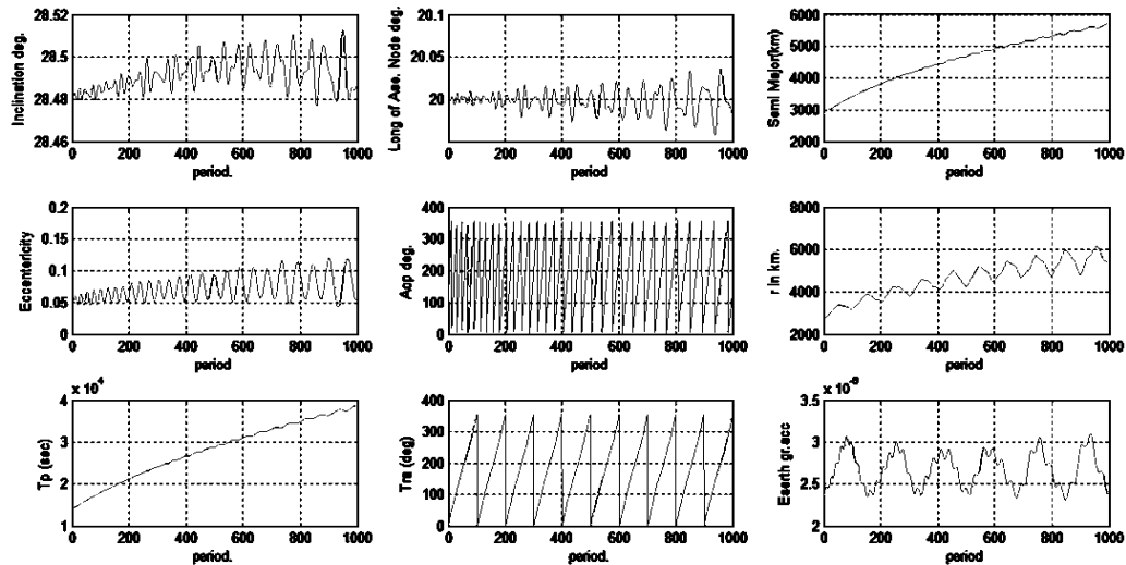
Figure 5 : The orbital elements variation at height=1000km.
