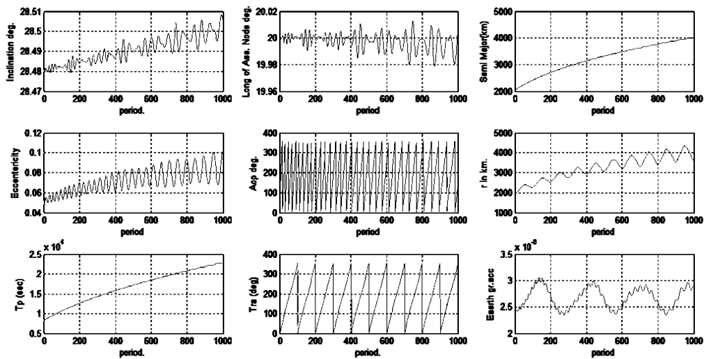
Figure 3 :The orbital elements variation at height=200km
