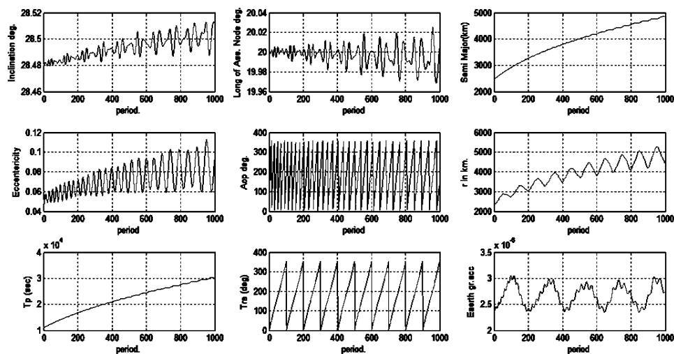
Figure 4 : The orbital elements variation at height=600km
