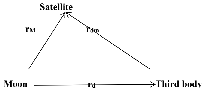
Figure 1: Definitions of third body attraction vectors.
