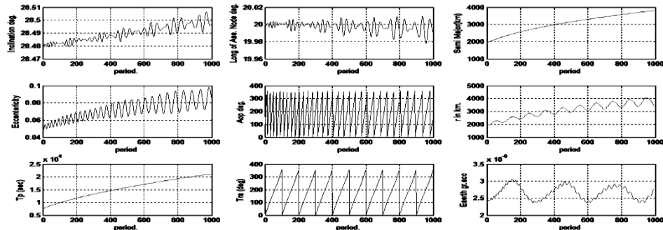
Figure 2 : The orbital elements variation at height=100km.
