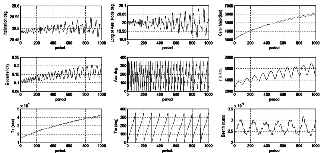
Figure 7 :Shows the orbital variation at height=1000km Case 1: e=0.05
