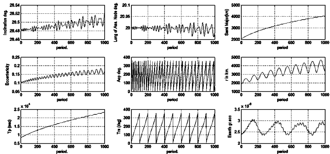
Figure 6 : Shows the orbital variation at height=100km
