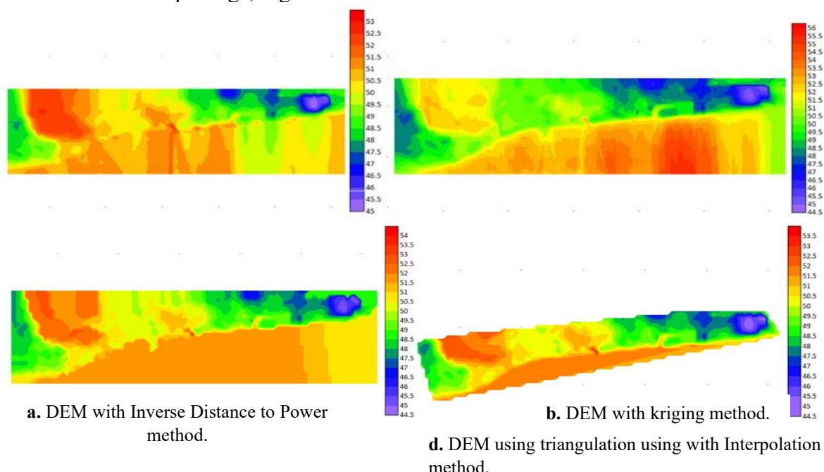
Figure 2: DEM using different methods (Prepared by Author).
