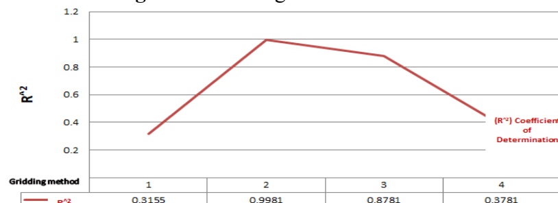
Figure 4: Gridding method VS R^2
