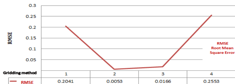
Figure 3: Gridding method VS RMSE
