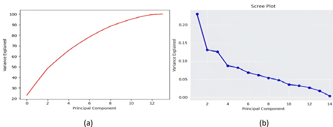
Figure 3: PCA: Principal Component Analysis (a) PCA plot (b) PCA-scree plot
