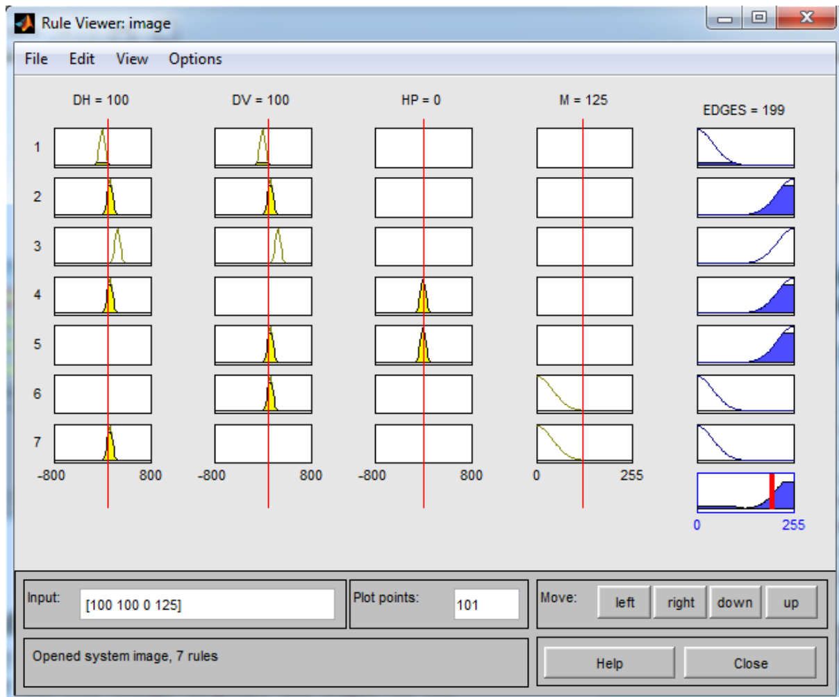
Figure 2- Proposed Fuzzy Inference System rule viewer.
