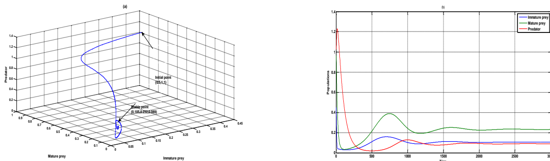
Figure. (6.1 ) (a) The solution approaches to E_2 = (0.105,0.232,0.089) (b) The time series of the attractor in Figure. (6.1a).
