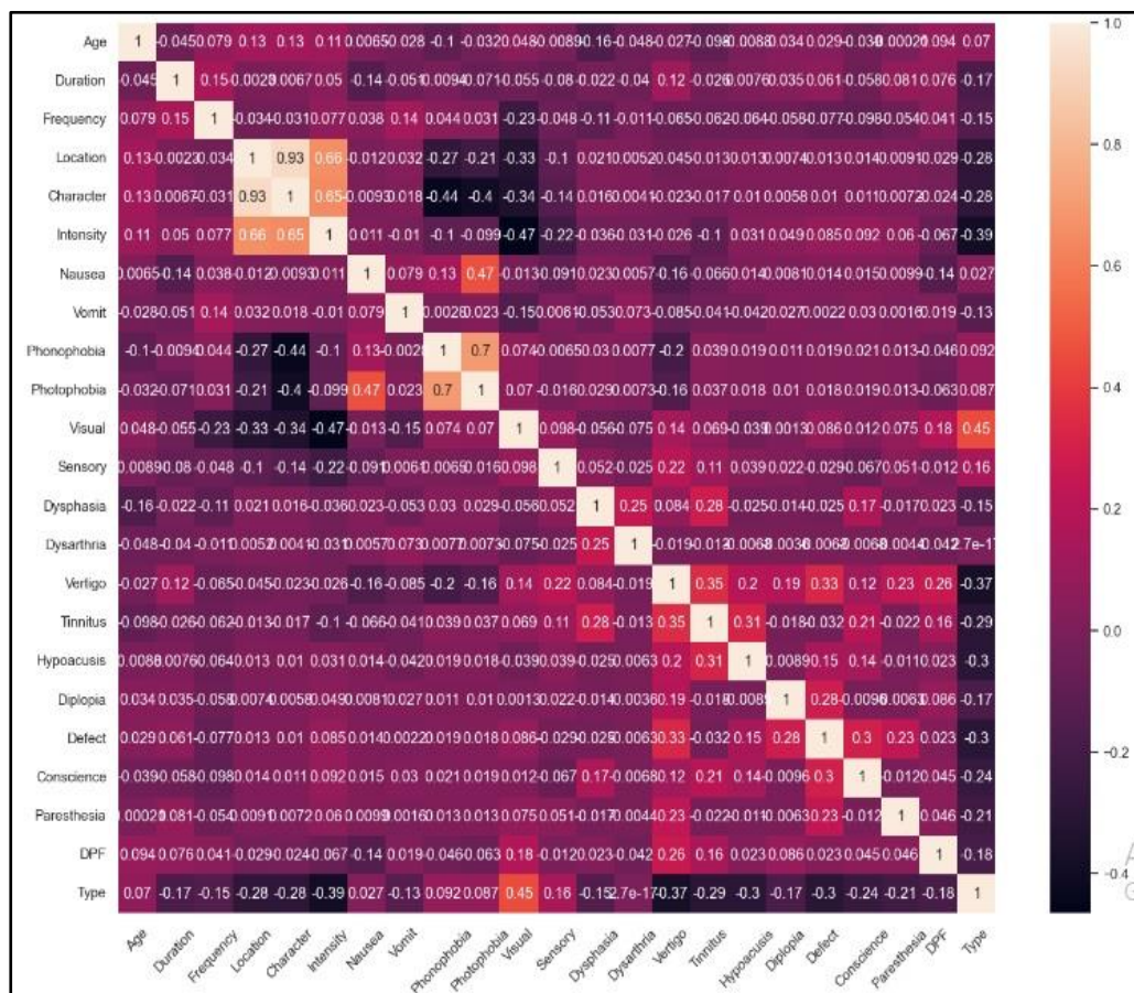
Figure 2: Correlation heatmap revealing the degree of relationship between variables
