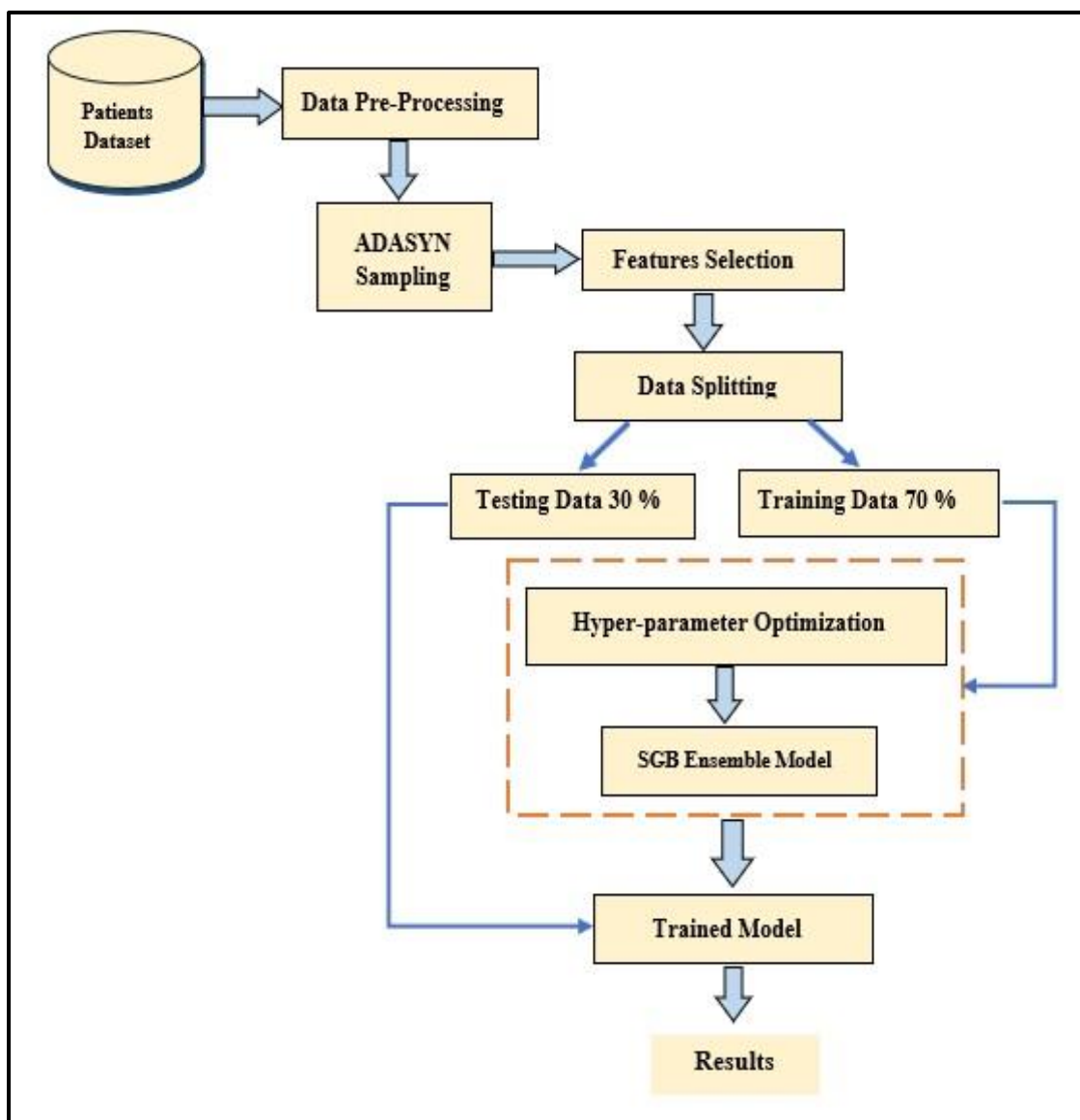
Figure 1: The Presented Work Architecture
