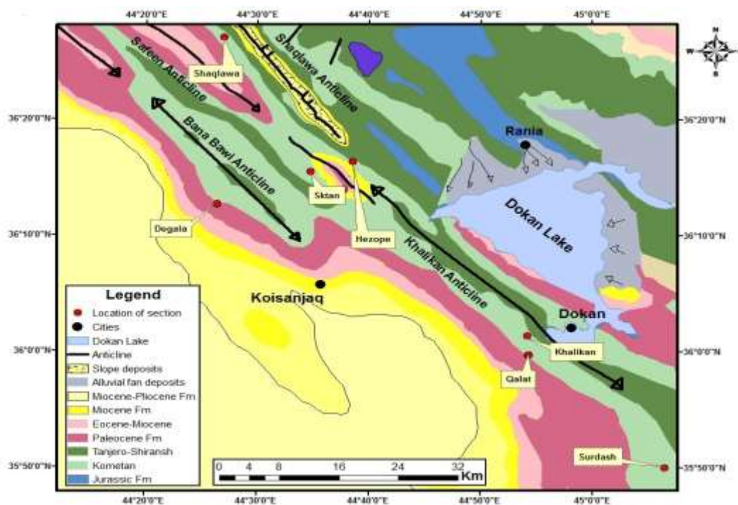
Figure 1- Geological and location map of studied area
